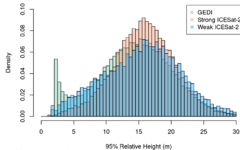
Figure 2. Histogram of the 95th percentile of relative height of the forested canopy over the Minnesota study area, as compared between GEDI and ICESat-2.
